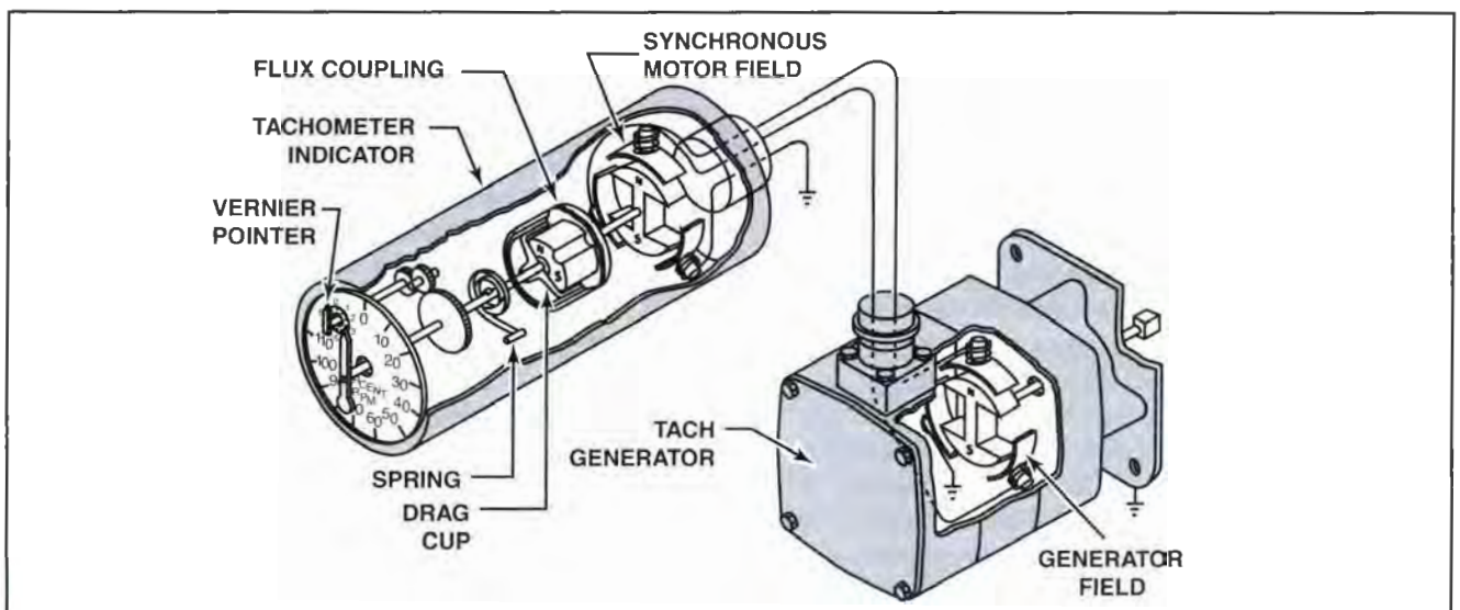
Figure 2-20. A typical electric tachometer consists of a three phase AC generator mounted on the engine accessory case and a synchronous motor in the indicator. The tach generator is driven by the accessory gearing in a running engine and produces an AC voltage at a frequency directly proportional to engine. The synchronous motor in the indicator is, in turn, driven by the AC voltage from the tach generator at the same speed, or frequency. The motor spins a drag cup assembly to move the instrument pointer.
