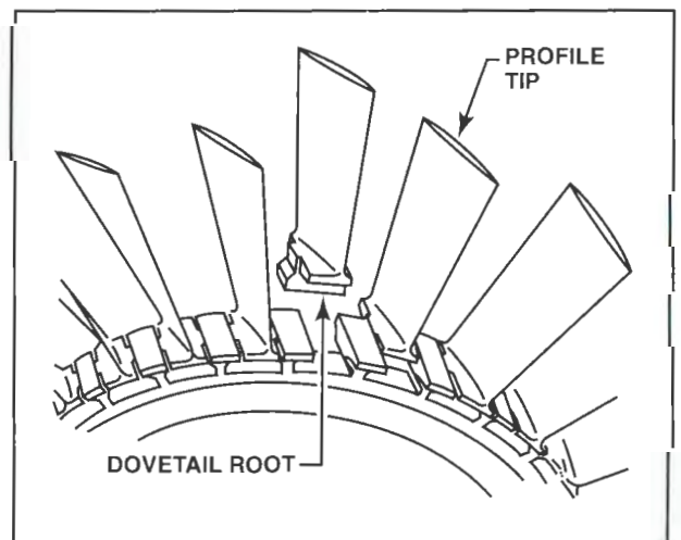
Figure 3-32. A dovetail on the base of this compressor blade fits loosely into a dovetail slot in the compressor wheel. A small locking device such as a pin, key, or plate prevents the blade from backing out.
