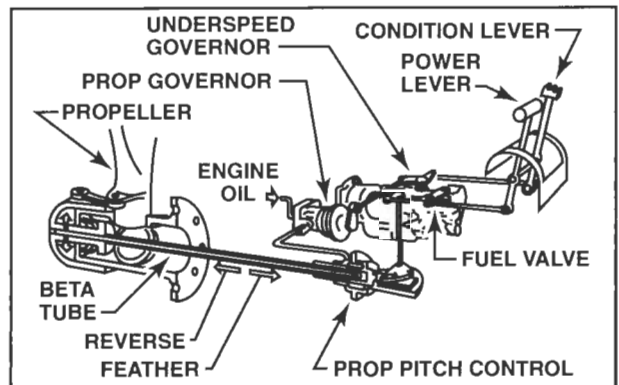
Figure 12-48. TPE-331 turboprop controls include a power lever and a condition lever.
