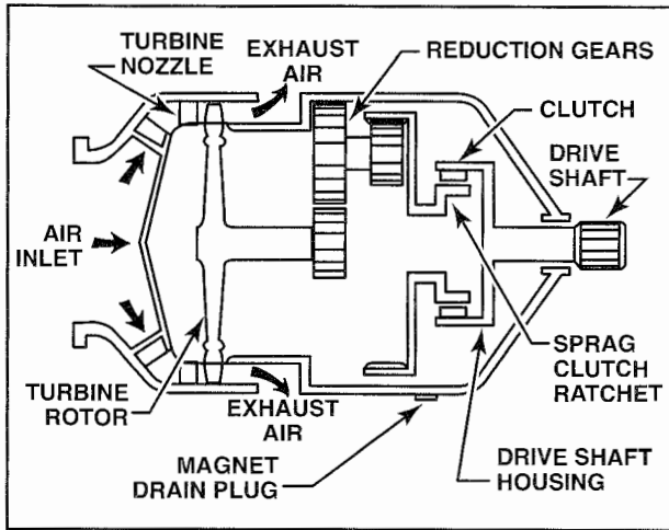
Figure 8-76. A typical air turbine starter consists of a small turbine assembly, reduction gearing, and a clutch assembly.
