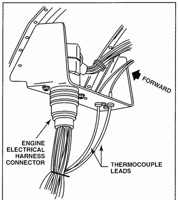
Figure 4-17. Most electrical connections are grouped in bundles and are disconnected at the firewall or junction by separating an AN or an MS electrical connector.
