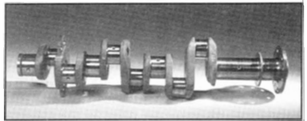
Figure 1-17. The crankpins in a typical six-throw crankshaft are 60 degrees apart in the firing order.
