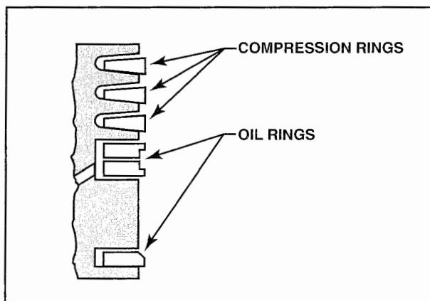
Figure 1-28. Compression rings are installed in the upper piston ring grooves to help prevent the combustion gases from escaping. Oil rings, on the other hand, are installed near the middle and bottom of a piston to control the amount of oil applied to the cylinder wall.
