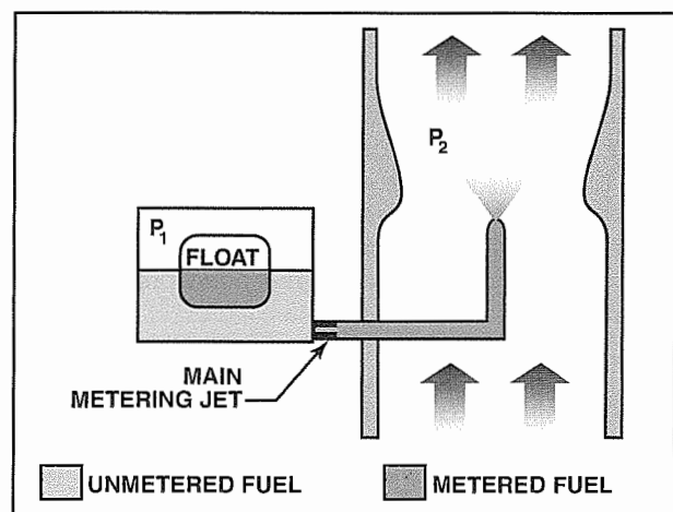
Figure 7-23. When intake air passes through the venturi, the pressure in the venturi ( P_2 ) is less than the pressure in the float chamber ( P_1 ). The pressure differential forces fuel from the discharge nozzle into the airstream. The greater the pressure differential between P_1 and P_2 , the greater the amount of fuel discharged.
