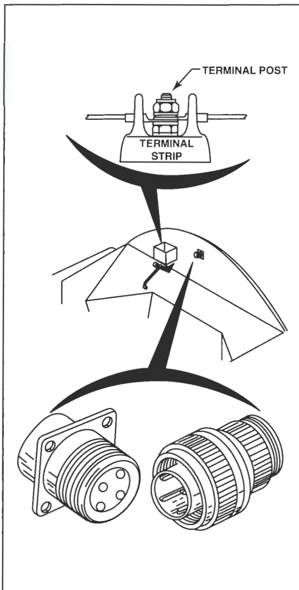
Figure 2-30. Aircraft that use firewall electrical disconnect points use two kinds of electrical connections. One type is a junction box containing terminal strips and terminal posts while the second type consists is a plug-type connector like a cannon plug or Amphenol connector.
