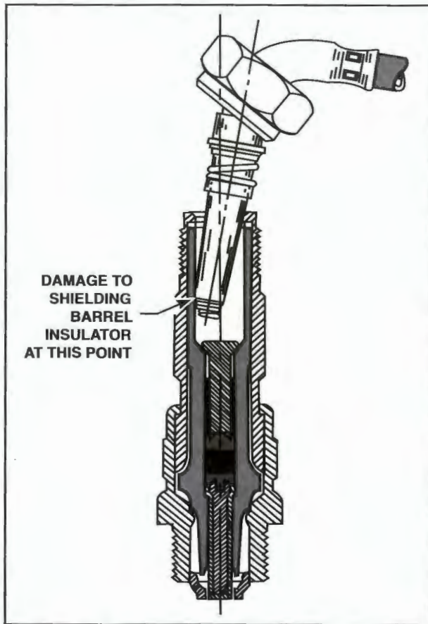
Figure 8-147. When removing the ignition lead from a spark plug, pull the terminal straight out of the plug. A side load on the ceramic insulator could cause a crack in the insulator.
