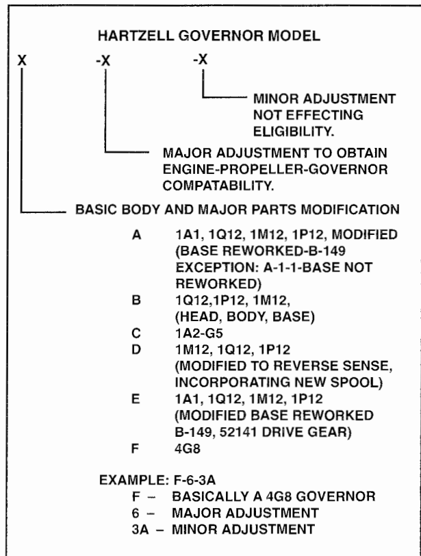
Figure 12-37. In the sample designation above, an F-6-3A propeller governor consists of a 4G8 governor with a major adjustment to obtain compatibility and a minor adjustment that does not affect its conformity to the original design.
