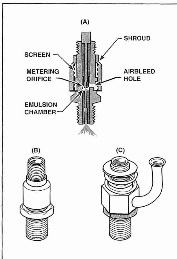
Figure 7-57 (A) A typical RSA fuel injector consists of a shrouded brass body housing a metering orifice, an air bleed hole, and an emulsion chamber. (B) The nozzles of normally aspirated engines are vented to ambient air that is drawn into the nozzle from under a shroud. (C) Because the manifold pressure in a turbocharged engine often exceeds atmospheric pressure, the nozzles on turbocharged engines accommodate a fitting to receive upper deck air pressure.
