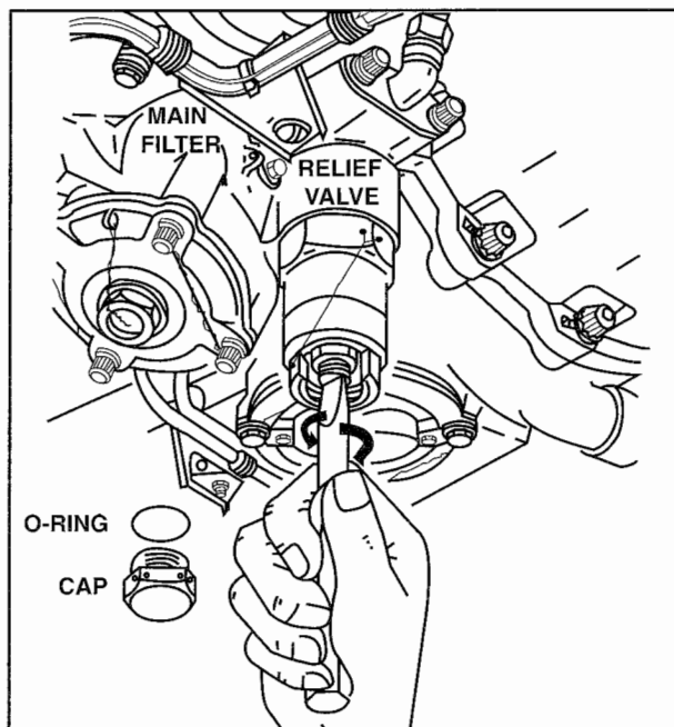
Figure 9-41. An oil pressure relief valve occasionally requires adjustment. With the engine operating at idle speed, turn the adjusting screw clockwise to increase oil pressure and counterclockwise to decrease oil pressure.
