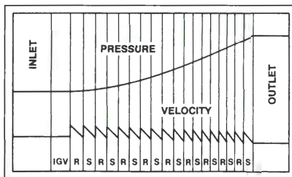
Figure 3-29. In an axial compressor, airflow velocity remains nearly constant as air pressure increases while air flows through each stage of compression.
