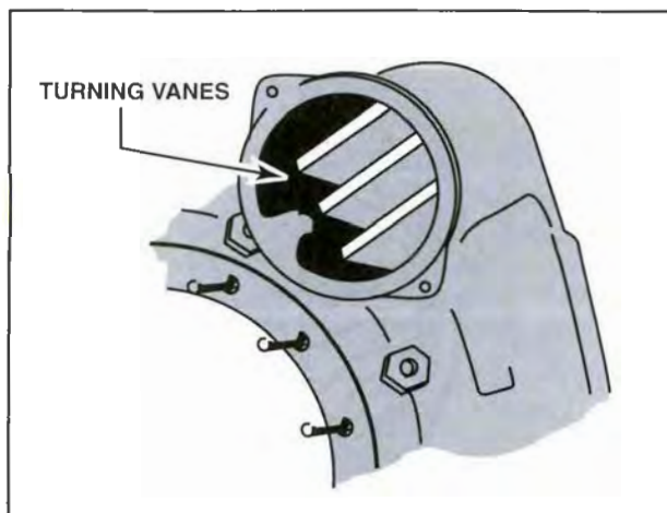
Figure 3-28. The turning vanes in a compressor manifold direct compressor outlet air to the combustion section.
