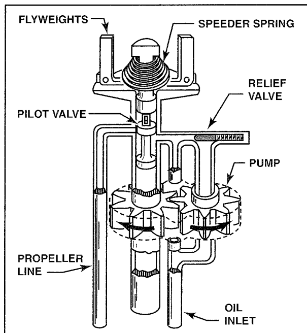
Figure 12-23. A typical propeller governor consists of a gear boost pump that increases oil pressure before it enters the propeller hub, a pilot valve that controls the amount of oil flowing into and out of the propeller hub, and a flyweight assembly that senses engine speed and positions the pilot valve to maintain a constant speed.
