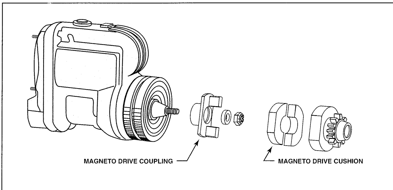
Figure 8-133. Some magnetos are connected to the engine with an anti-vibration coupling. The engine drives the magneto through a rubber cushion housed by a steel retainer attached to the magneto drive gear. The cushion reduces the amount of vibration transferred to the magneto.
