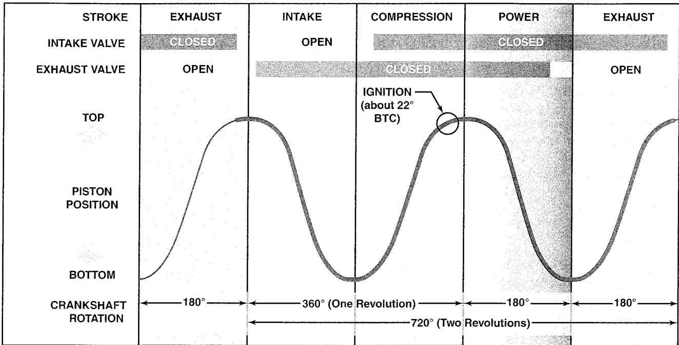
Figure 1-60. This timing diagram shows piston and valve positions during the four strokes of the Otto cycle. The bold line indicates that the five events (intake, compression, ignition, power, and exhaust) do not perfectly align with the four strokes (intake, compression, power, and exhaust).
