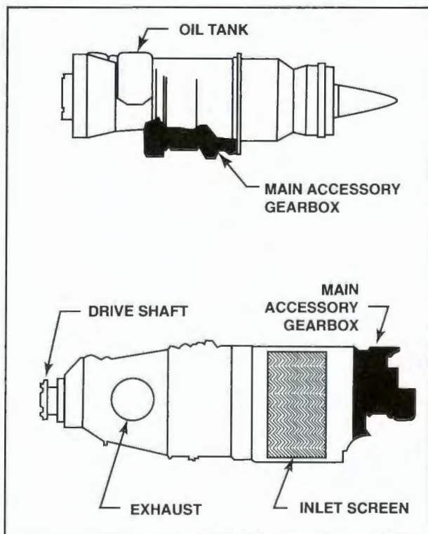
Figure 3-58. Accessory drives typically blend with the engine profile to minimize drag.
