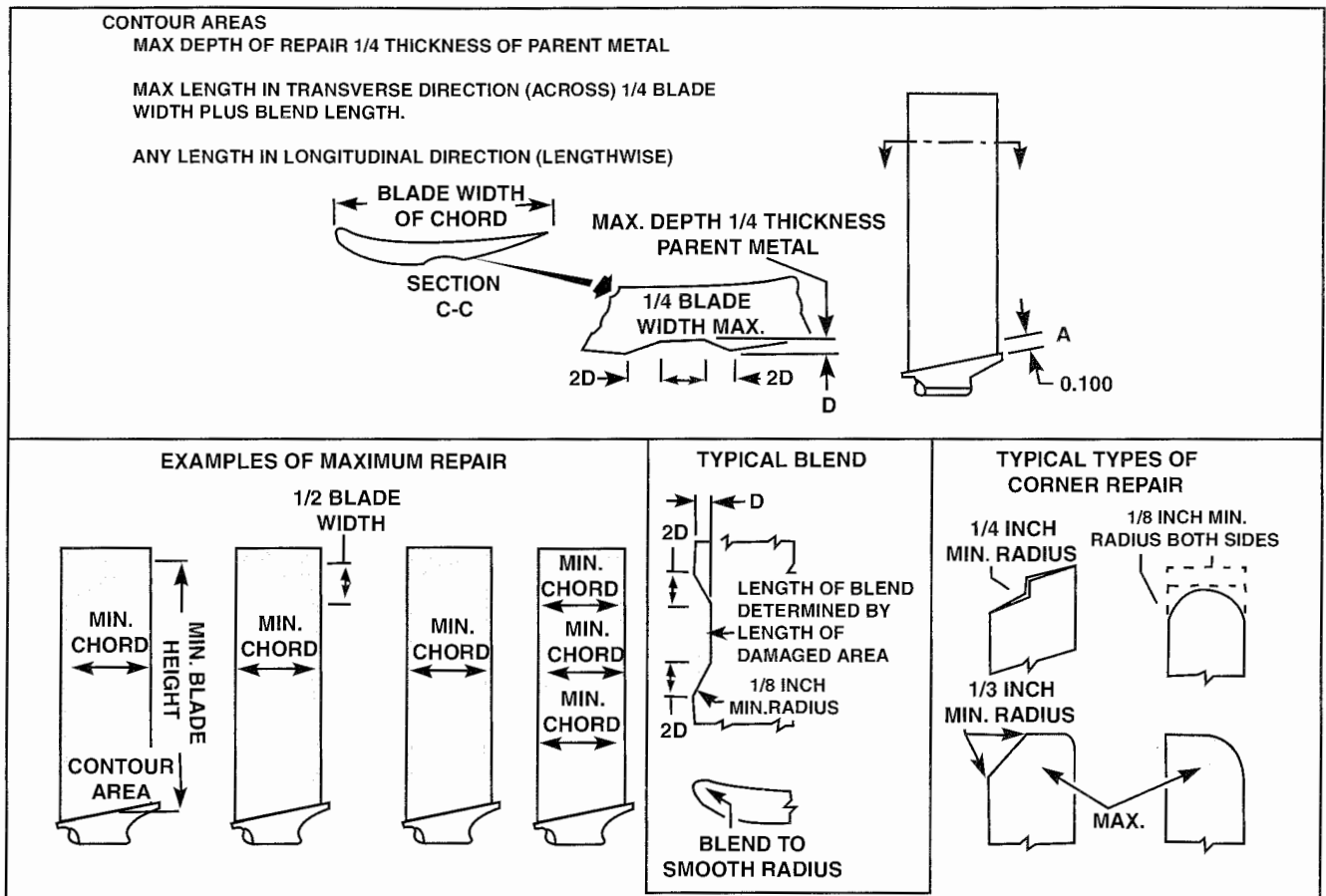
Figure 4-29. Compressor blade repairable limits and blended repairs are based on blade width, length, and chord dimensions. Typically, most leading and trailing edge damage as well as tip damage is repairable provided you maintain a minimum chord and height.
