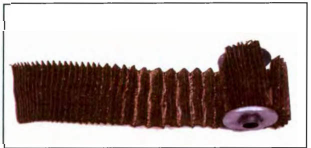
Figure 13-16. When changing oil during an inspection, the oil filter should be opened so you can check for metal particles or other contamination.
