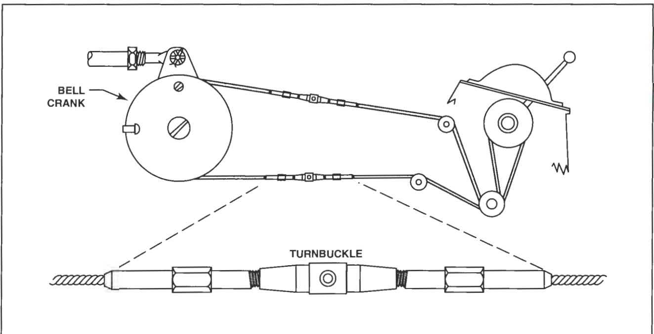
Figure 2-32. Some control systems consist of a cable and pulley arrangement to actuate engine controls. With this style of system, the cable assembly may have to be separated at a turnbuckle in order to remove the control rod.
