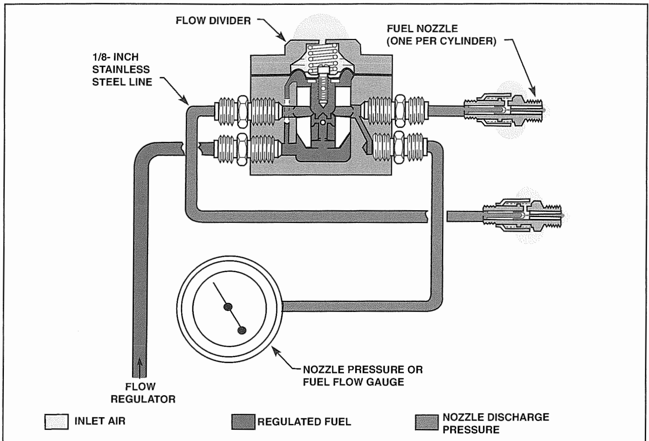
Figure 7-56. A flow divider ensures equal fuel flow at a regulated pressure to each nozzle. In addition, it provides a convenient location to take a system pressure reading. A pressure gauge connected to the flow divider can be calibrated to display fuel flow.
