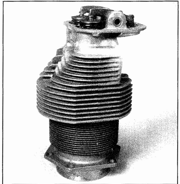
Figure 1-31. The cylinder assembly, the piston assembly, connecting rods, crankshaft, and crankcase constitute the power section of a reciprocating engine.
