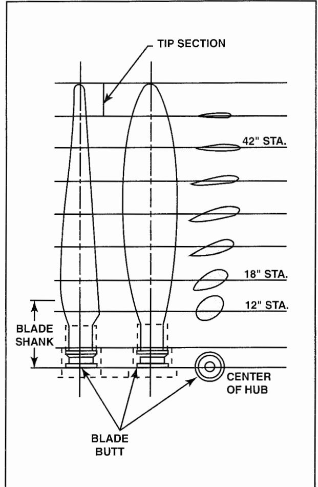
Figure 12-8. The variation in airfoil shape and blade angle along the length of a propeller blade compensates for differences in rotational speed and provides a relatively even distribution of thrust along the blade.
