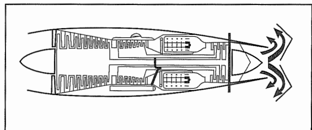
Figure 6-10. Thrust reversers change the direction of exhaust gas flow from a rearward to a more forward direction. This illustration shows a mechanical blockage thrust reverser.
