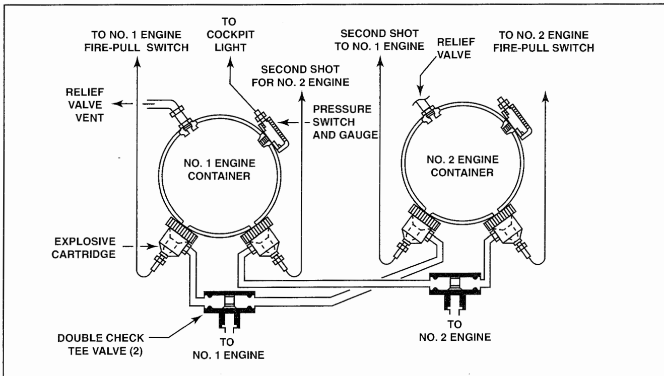
Figure 11-22. A typical high-rate discharge extinguishing system on a large multiengine aircraft uses two agent containers, each with two discharge ports. This permits two applications of extinguishing agent to any one engine.
