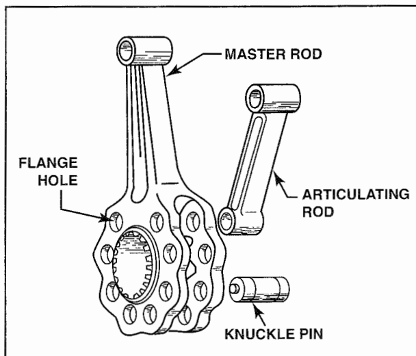
Figure 1-21. Articulated rods are attached to the master rod by knuckle pins. A knuckle pin lock plate retains the pins.
