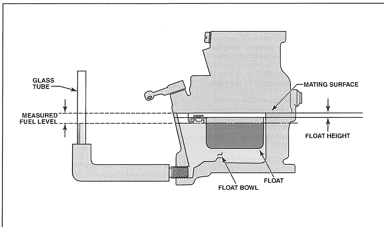
Figure 7-39. After you mark a line level with the carburetor's parting surface on a sight glass, measure the distance between the fuel level and parting surface. This check verifies the correct fuel level and the proper functioning of the float and needle valve assembly.
