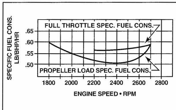
Figure 1-72. Aircraft engines tend to operate most efficiently around 2,400 r.p.m. Below this speed, an engine does not develop maximum power for the amount of fuel it is using. Above 2,400 r.p.m., friction horsepower increases, causing an overall drop in brake horsepower. A typical engine requires about 0.51 pounds of fuel per hour for each horsepower it produces at 2,400 r.p.m.
