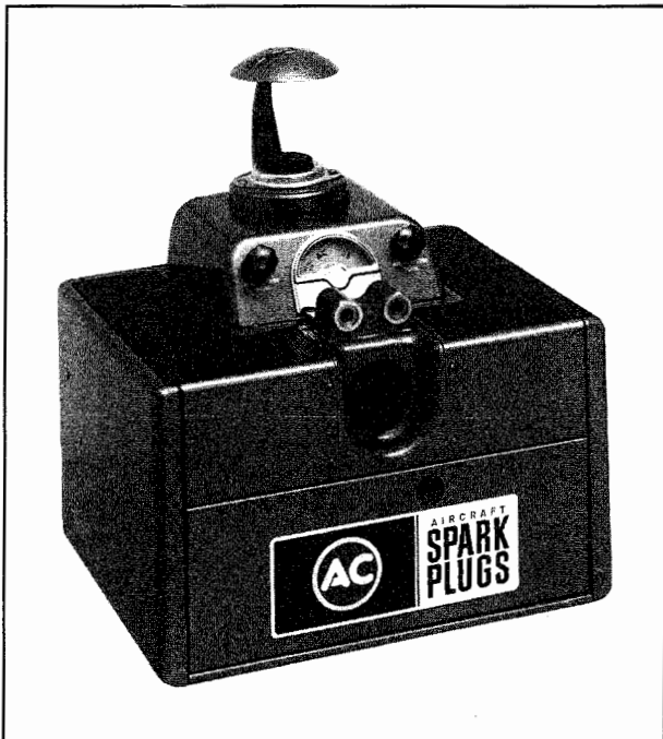
Figure 8-156. A combination spark plug cleaner and tester is widely used in maintenance shops.
