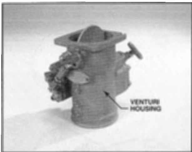
Figure 7-49. A typical venturi housing is a single piece of cast aluminum with a venturi pressed into one end. A throttle valve is installed on the other end.
