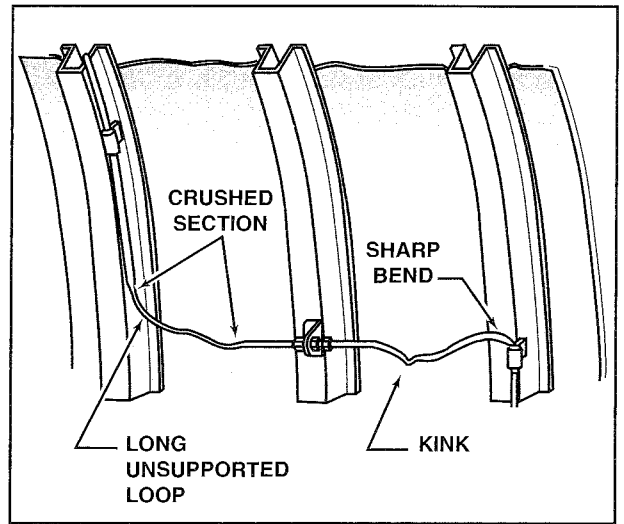
Figure 11-14. Fire sensing elements are located in exposed areas and are subject to impact and abrasion. When inspecting fire elements, look for sharp bends, kinks, and crushed sections.
