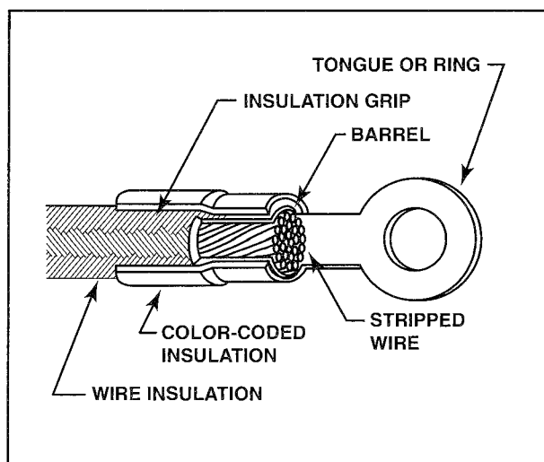
Figure 8-92. Wire gauge sizes 10 through 22 are typically terminated with preinsulated, solderless terminals that are color-coded to identify size.
