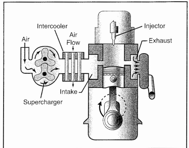
Figure 1-78. Two stroke diesel engines can be supercharged and intercooled to increase performance.
