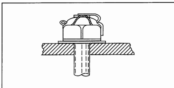
Figure 12-97. If the propeller installation uses castellated nuts with drilled bolts, safety the nuts with cotter pins.
