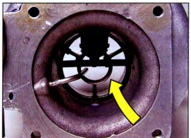
Figure 14-9. A loose venturi produces turbulence in the intake which can cause engine hesitation during acceleration.
