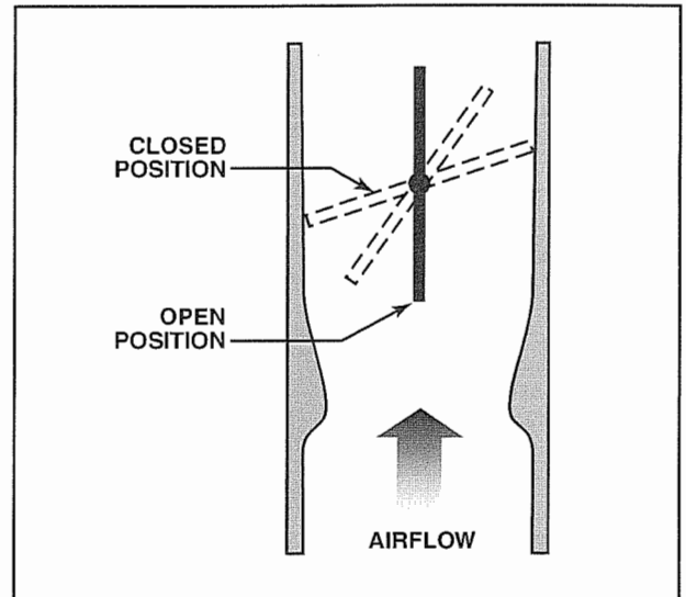
Figure 7-20. When the throttle valve is parallel to the airflow, the maximum volume of air and fuel enters the engine. When the throttle valve is near perpendicular to the airflow, less air and fuel enter the engine.
