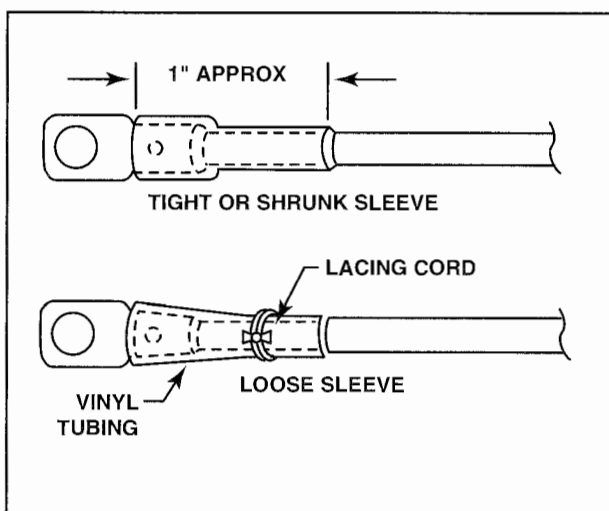
Figure 8-93. Solderless terminals installed on 10-gauge or larger wire require a separate piece of insulation. You can use heat-shrinkable tubing or vinyl tubing secured with lacing cord.
