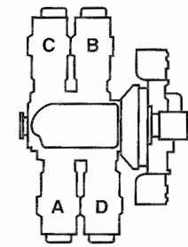
CONTINENTAL FOUR-CYLINDER ENGINE
