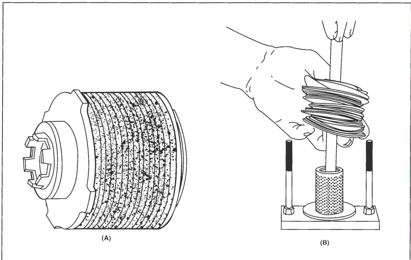
Figure 9-35. (A) A typical screen-disk filter consists of several wafer-thin screens separated by spacers. (B) This configuration allows easy disassembly and cleaning.
