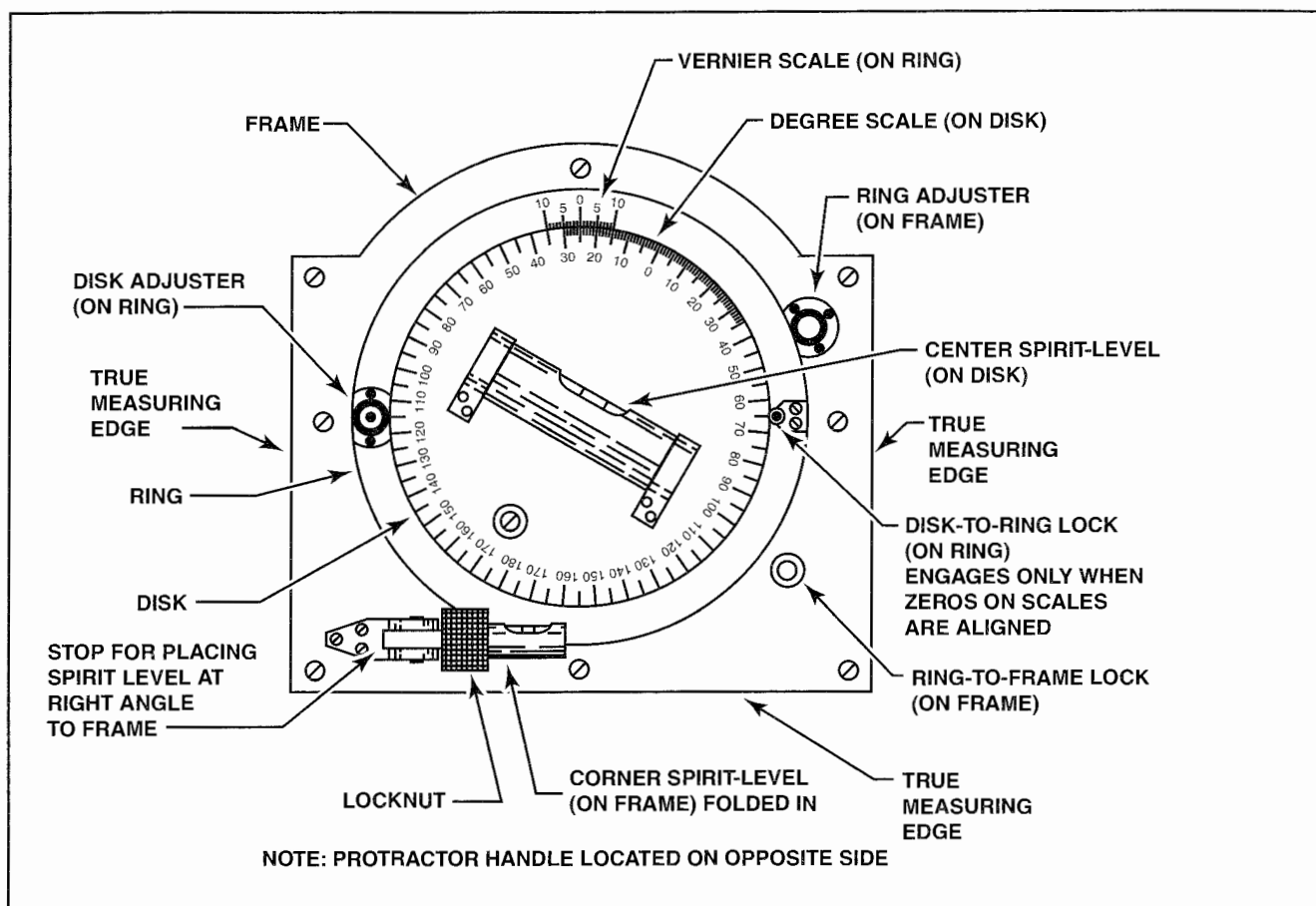
Figure 12-74. A universal propeller protractor is used to check propeller blade angle.
