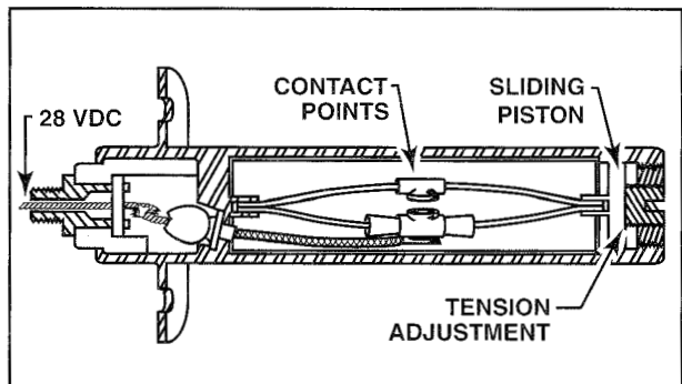
Figure 11-1. The sensor on a thermal switch detector is mounted inside a stainless steel housing. In a fire, the housing heats up and becomes elongated, which causes the contact points to close. To adjust a thermal switch, heat the housing to the specified temperature and adjust the tension screw until the contacts just close.
