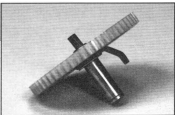
Figure 8-119. In a typical magneto, a small carbon brush routes current to the distributor rotor. From the distributor rotor, current passes to the distributor block through a distributor finger.
