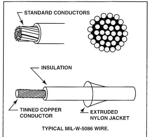
Figure 8-81. MIL-W-5086 wire consists of stranded copper conductors covered with tin and wrapped with PCV insulation. For added protection, a nylon coating often covers the wire.
