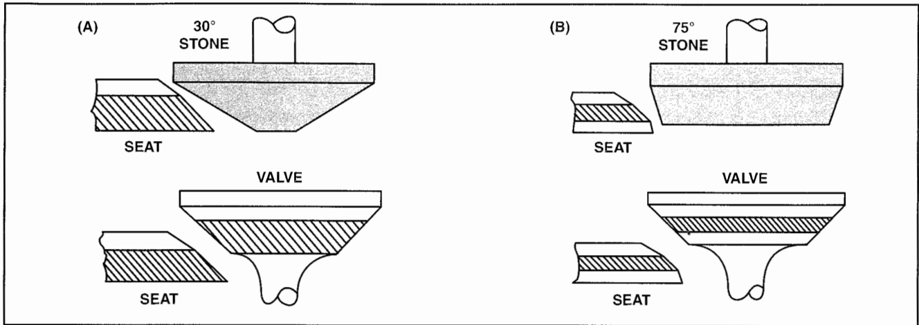
Figure 2-63. (A) If a valve seat contacts the upper third of the valve face, the seat can be regrouned to a lesser angle. (B) Contact with the bottom third of the valve face requires regrinding a valve seat's inner corner to a greater angle.
