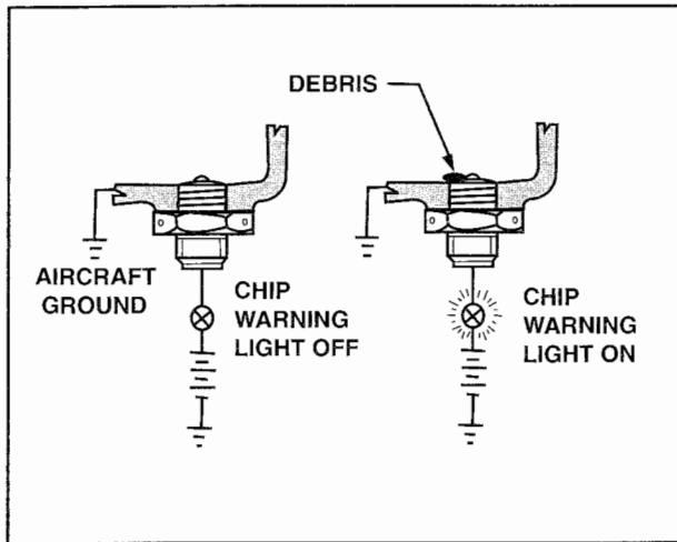
Figure 9-38. With a chip detector that incorporates a warning light, ferrous debris collecting on the magnet bridges the gap between the positive and ground electrodes and completes the indicating circuit.
