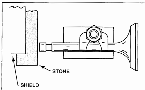
Figure 2-60. To accurately grind a valve tip, the valve must be held securely in place and be aligned perpendicular to the side of the grinding stone.
