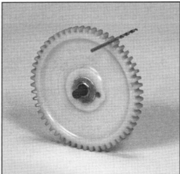
Figure 8-127. To check for excessive wear between distributor gear teeth, insert a specific size drill bit between the teeth. If the bit fits snugly, the gear is within specifications.
