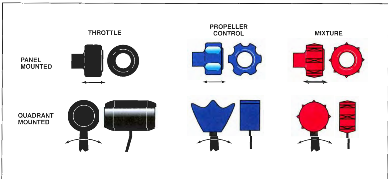
Figure 2-1. For standardization purposes, the primary engine controls are arranged from left to right beginning with the throttle, propeller control, and mixture. In addition, each lever is color-coded and uniquely shaped.
