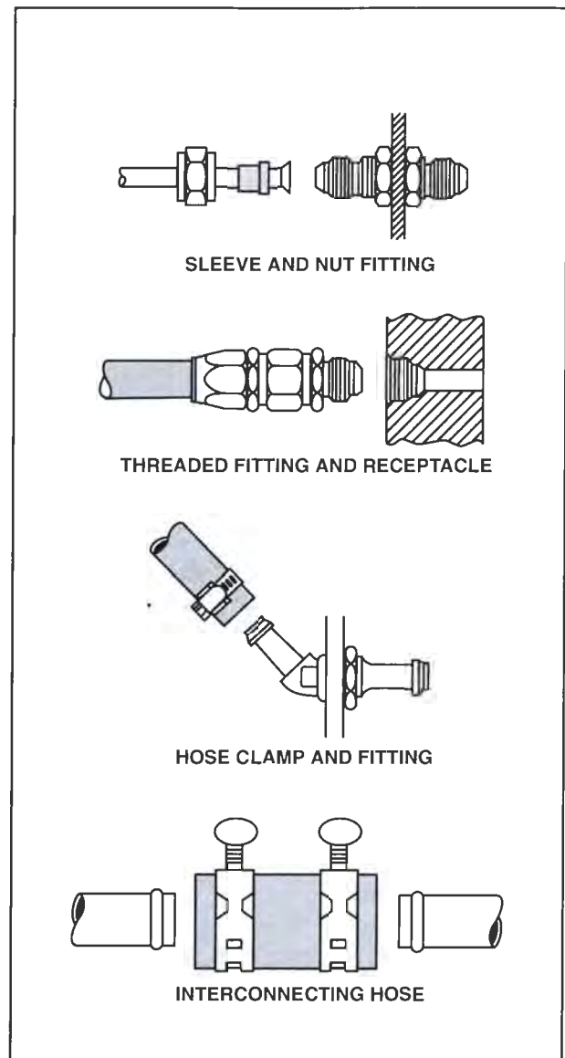
Figure 2-29. Fluid lines are typically connected to the firewall or an accessory by a B-nut, a threaded fitting and a receptacle, or hose clamps.
