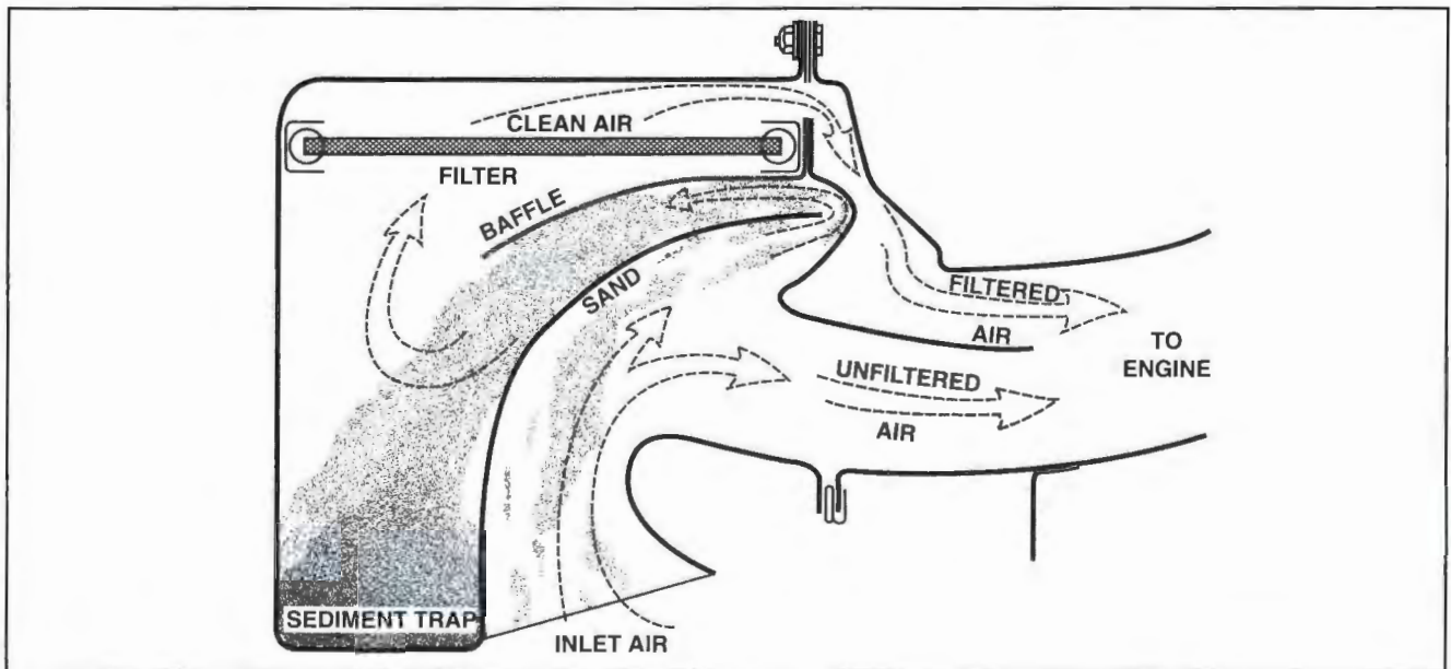
Figure 3-22. Sand and dust separators are typical for a turbine-powered helicopter. The venturi in the air inlet accelerates air and sand, but because the sand has too much inertia, it cannot make the turn leading to the engine.
