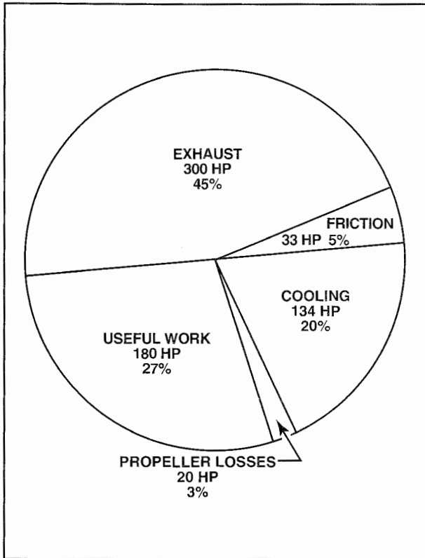
Figure 1-73. The distribution of power from aviation gasoline consumed by a typical 200 horsepower engine.
