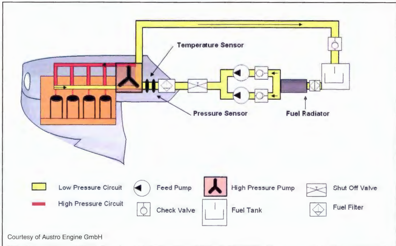
Figure 7-69. The fuel system of the Austro AE300 is illustrated with this schematic from the operating manual.
