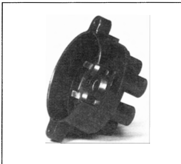
Figure 8-120. The distributor block of a typical magneto is made of an insulating material with electrodes on one side and receptacles for spark plug on the other.
