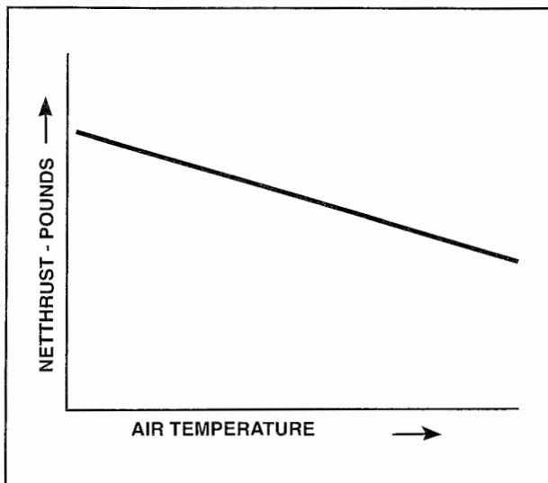
Figure 3-72. Air density decreases as temperature rises; the lower the density of the air, the less thrust an engine can produce.
