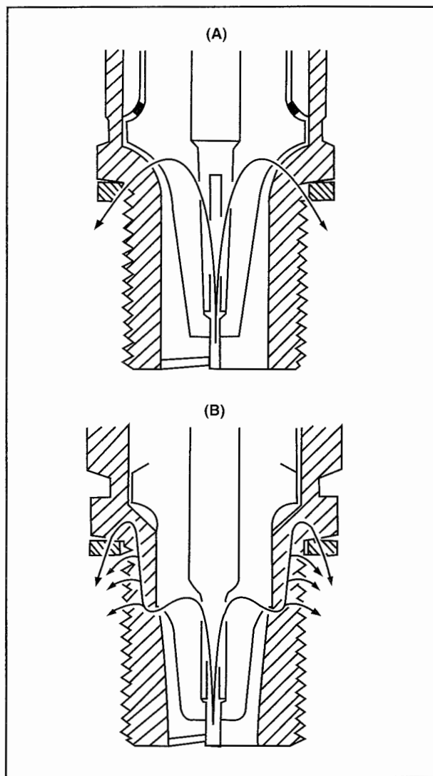
Figure 8-146. (A) Hot spark plugs have long nose cores that provide relatively little contact area between the insulator and shell. The small amount of contact area slows the rate at which heat can be conducted away from the plug tip. (B) Cold plugs, on the other hand, have a shorter nose core that permits a large contact area for dissipating heat.
