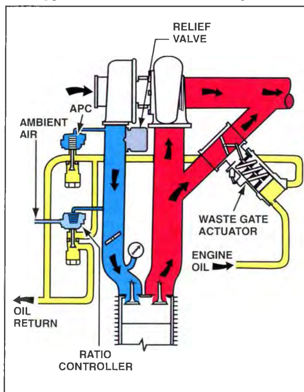
Figure 5-14. On turbocharging systems that are restricted to a maximum differential between manifold and ambient pressures, a pressure ratio controller is installed in parallel with the absolute pressure controller in the oil line between the wastegate actuator and the engine sump.
