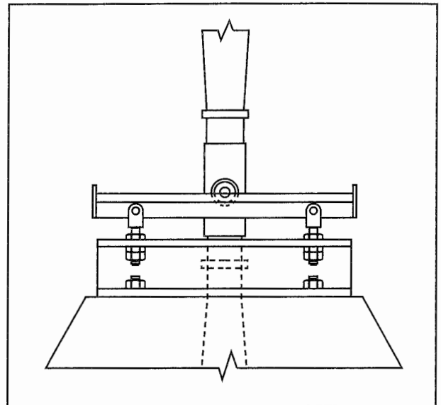
Figure 12-71. In a vertical balance check, the propeller blades are aligned vertically and an imbalance condition causes them to rotate.
