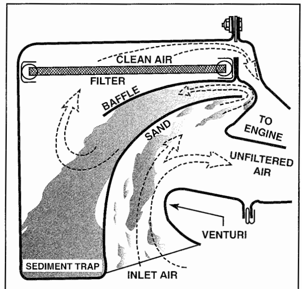
Figure 5-30. This particle separator is typical of the type found on turbine-powered helicopters. The venturi in the air inlet accelerates the air and sand, so the sand has too much inertia to make the turn leading to the engine.
