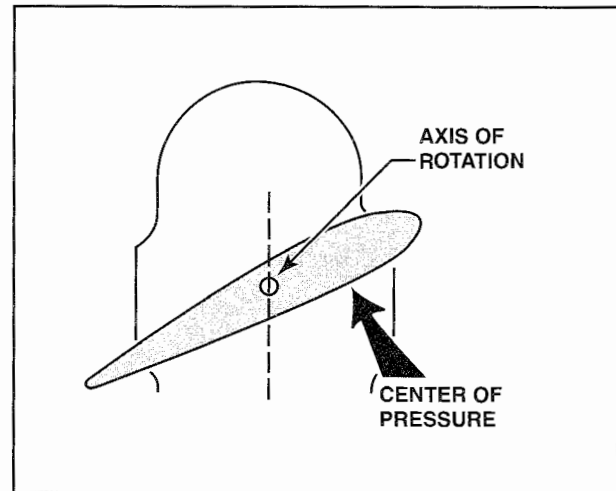
Figure 12-12. The majority of thrust produced by a propeller is exerted ahead of the blade's axis of rotation. This produces an aerodynamic twisting force that tends to increase propeller blade angle.
