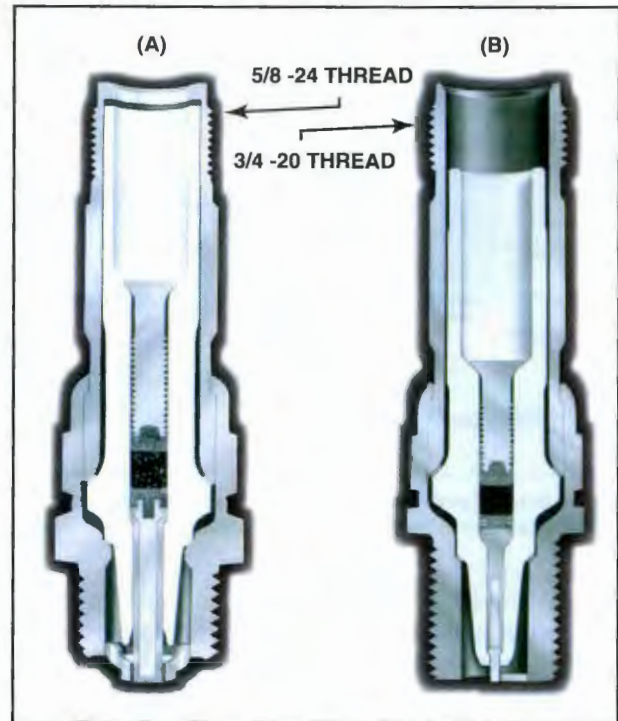
Figure 8-144. (A) The 5/8-24 thread is often used on older massive-electrode spark plugs. (B) The 3/4-20 thread is most often used with all-weather spark plugs. With all-weather spark plugs, the ceramic insulator is recessed in top of the shell with room for a resilient grommet on the ignition lead to form a watertight seal.
