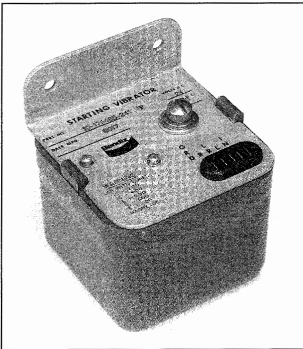
Figure 8-125. The typical vibrator unit consists of several solid state components sealed in a case and mounted to aircraft structure.
